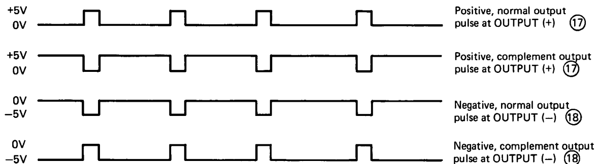
Figure 3-2. Normal/Complement Outputs
