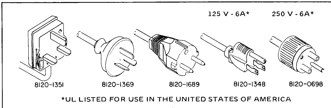
Figure 2-2. Power Cables.
