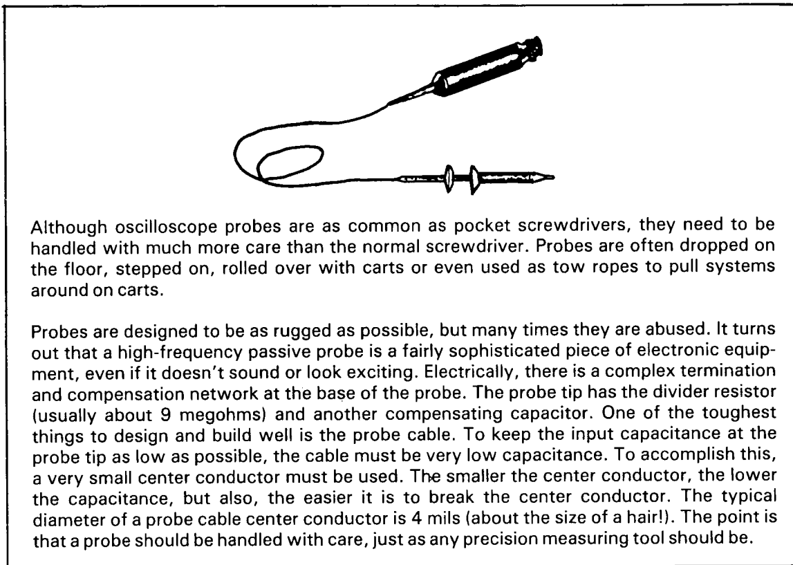
Figure 3-25. About Scope Probes.
