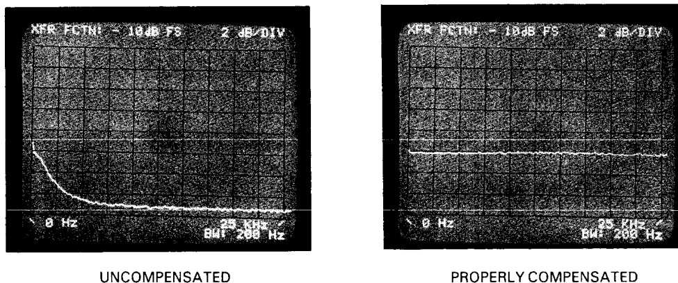
Figure 3-26. Probe Compensation.
