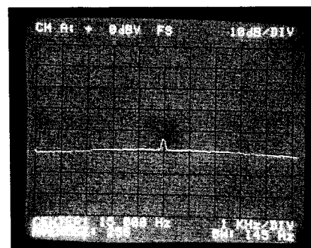
Figure 3-19. RMS Averaged Signals.
