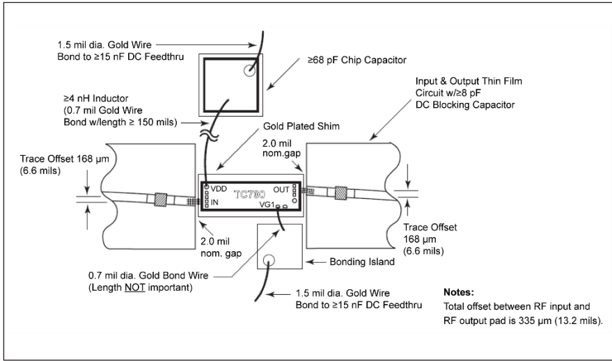
Figure 3. Assembly diagram (For 2 – 26 GHz operation).
