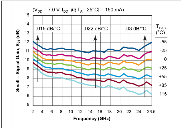
Figure 6. Sample small signal gain vs. temperature.
