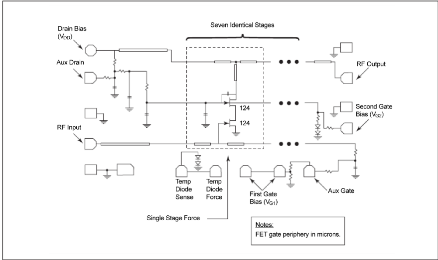
Figure 1. Schematic.
