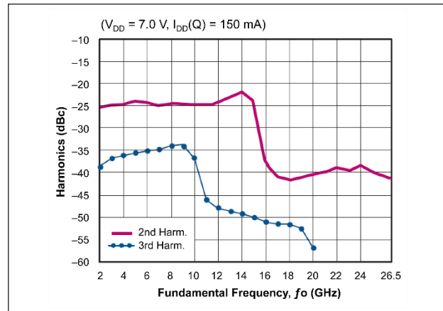
Figure 9. Sample 2 nd and 3 rd harmonics vs fundamental frequency at P_{out} = +17\text{ dBm} .
