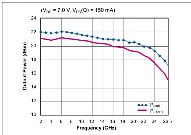
Figure 8. Sample 1dB gain compression and saturated output power.
