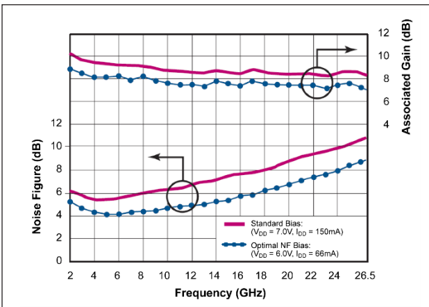
Figure 10. Sample noise figure performance.
