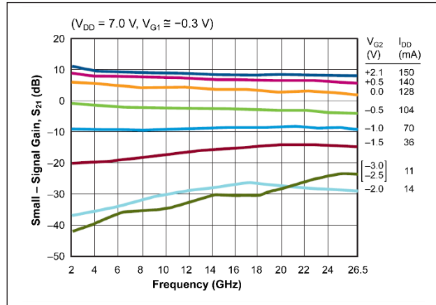
Figure 7. Sample gain vs second gate control voltage.
