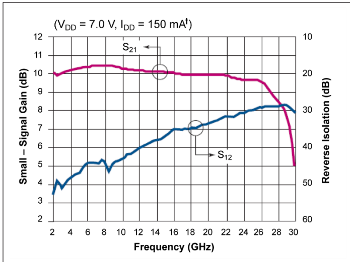
Figure 4. Sample Gain and reverse isolation vs frequency.
