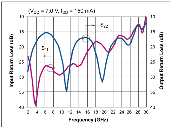
Figure 5. Sample input and output return loss vs frequency.
