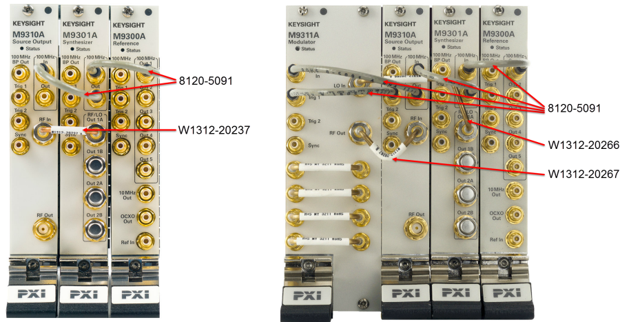
Keysight M9380A PXIe CW Source
