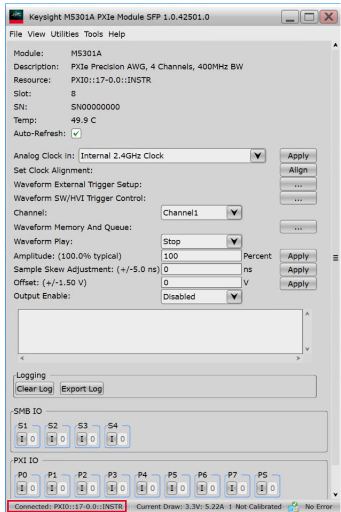
Figure 35 “Connected to <VISA address>” in the status bar on the main window
