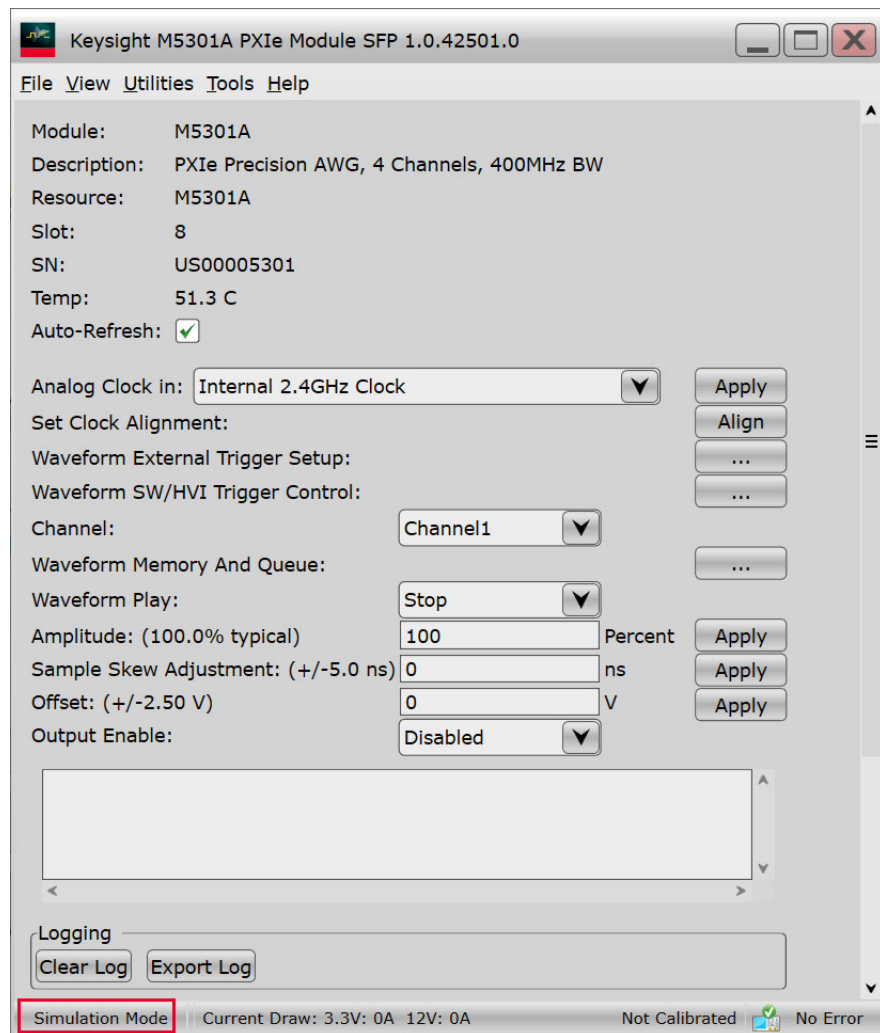
Figure 33 “Simulation Mode” in the status bar on the main window
