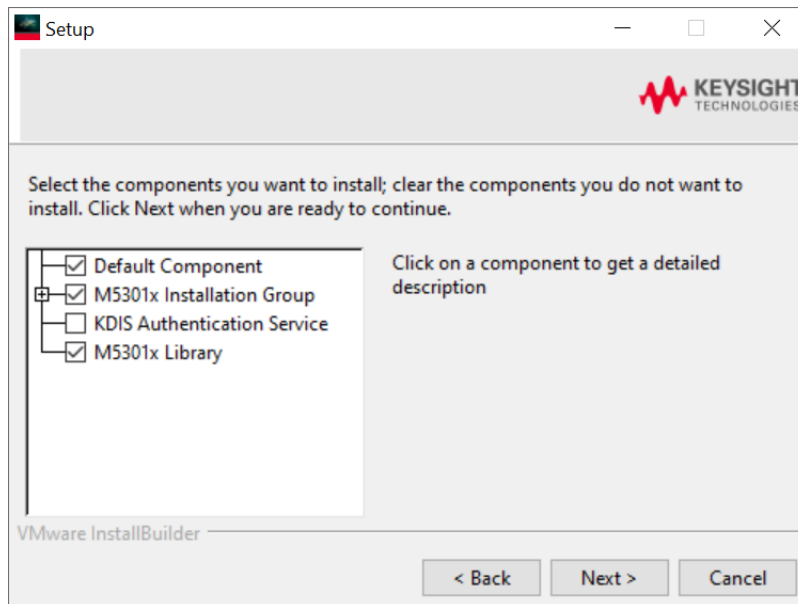
Figure 24 Selecting / clearing components during M5301x SW installation
