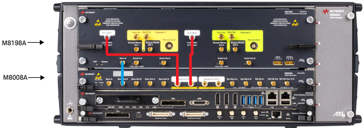
Figure 16 Connecting M8008A clock generator to two channels of M8198A AWG
