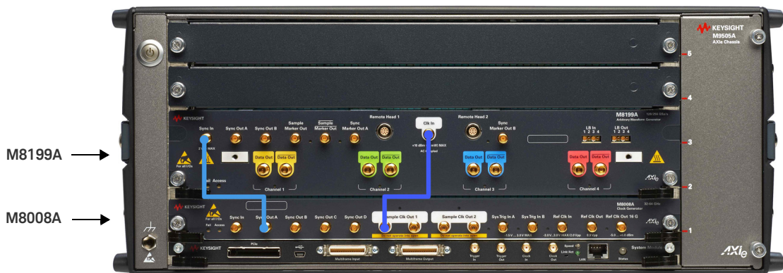
Figure 17 Connecting M8008A clock generator to M8199A AWG module
