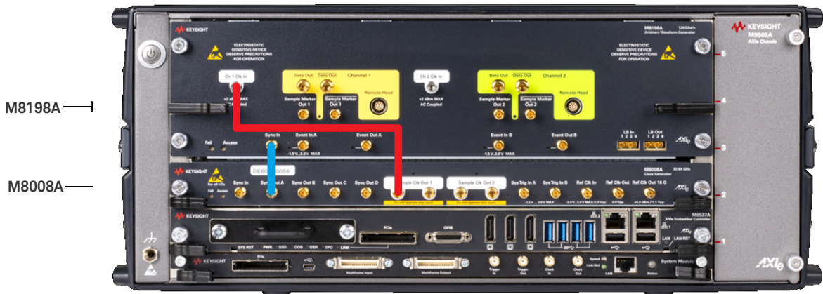
Figure 15 Connecting M8008A clock generator to a single channel of M8198A AWG
