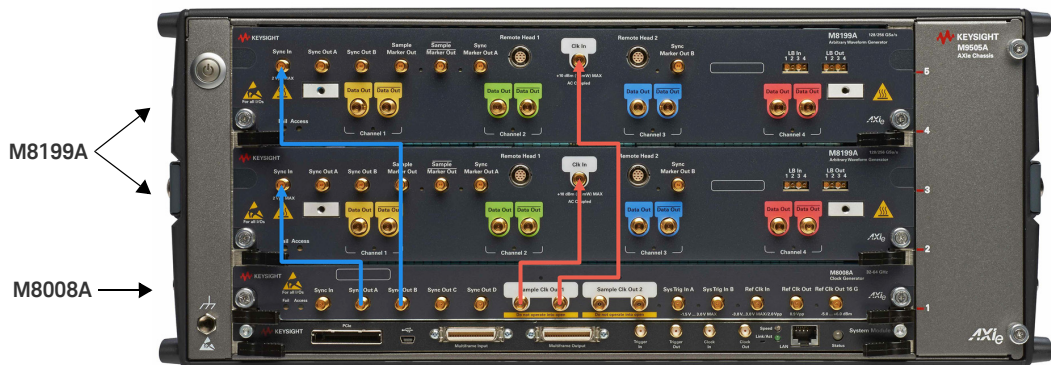
Figure 18 Connecting M8008A clock generator to two M8199A AWG modules
