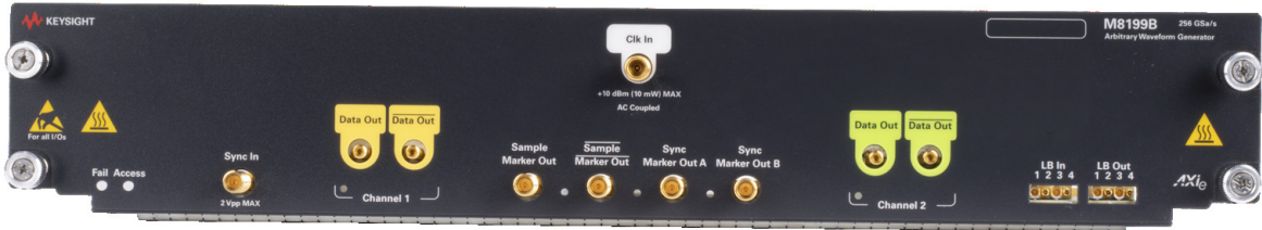
Figure 11 M8199B module front panel
