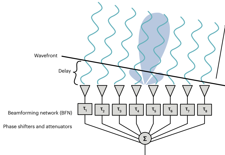
Figure 3. Varying the signal delay to each element shifts the individual wavefronts produced, which steers the beam. All the individual wavefronts combine to create a single wavefront propagating in the direction of the main beam from the antenna.
